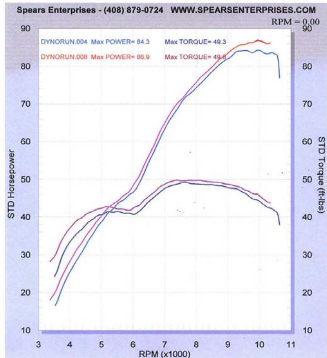
■ DYNORUN.004 Stock Suzuki Rotor, 3.2 LBS ro 4/18/06 5:34:10 PM ■ DYNORUN.008 Lighten rotor ro 10/9/06 6:29:02 PM
